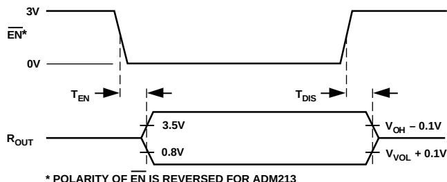
Figure 25. Enable Timing
