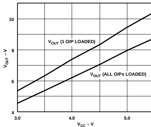
Figure 17. Transmitter Output Voltage vs. V_{CC}
