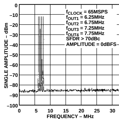
Figure 15. Four-Tone SFDR
