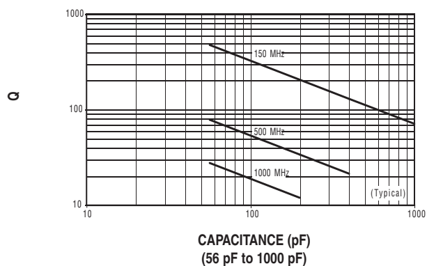
Q VS. CAPACITANCE ATC SERIES 100, CASE B
