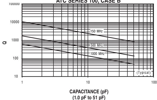
Q VS. CAPACITANCE ATC SERIES 100, CASE B
