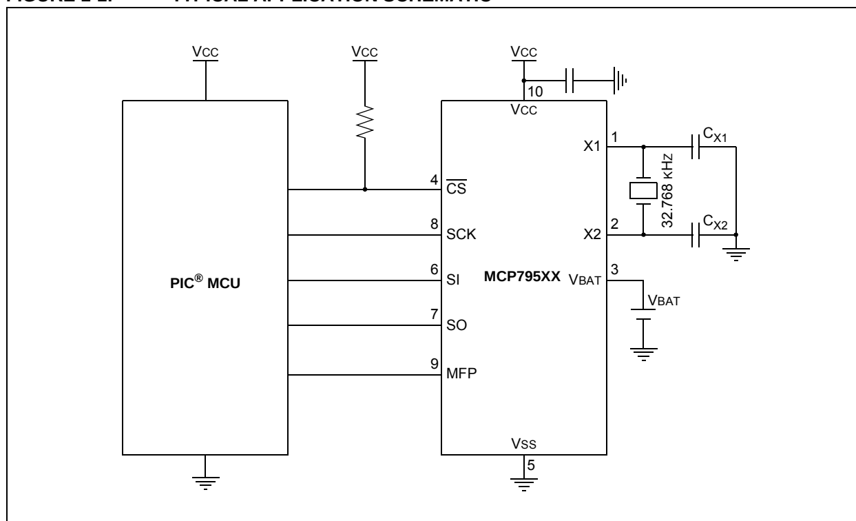
FIGURE 1-1: TYPICAL APPLICATION SCHEMATIC
