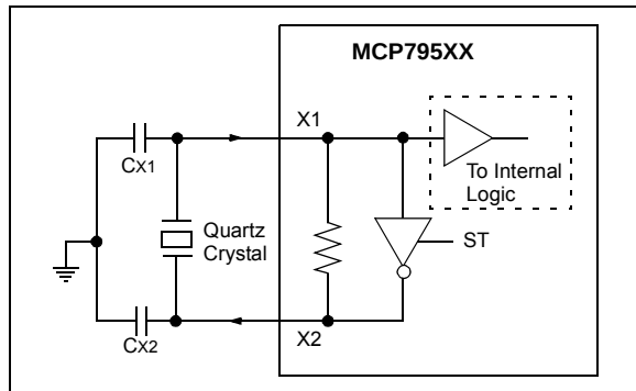
FIGURE 5-3: CRYSTAL OPERATION
