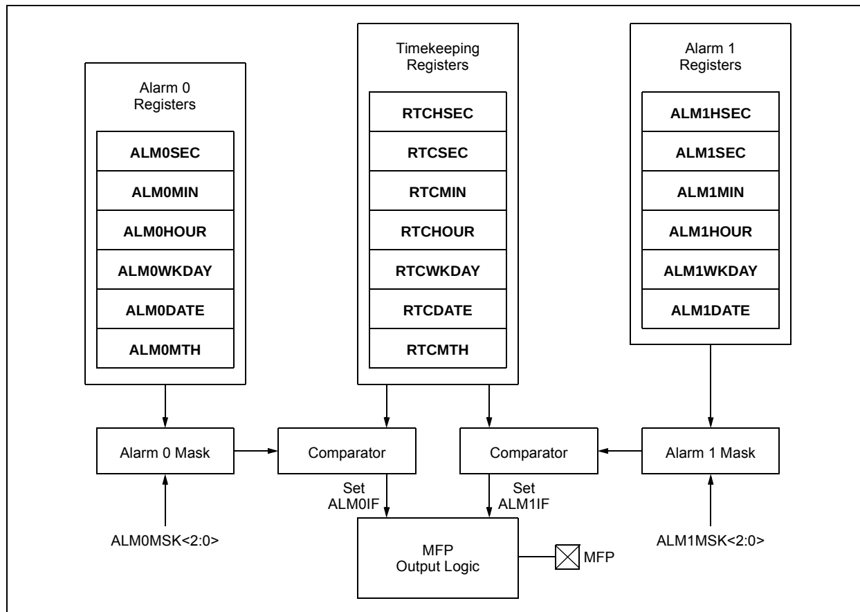
FIGURE 5-7: ALARM BLOCK DIAGRAM
