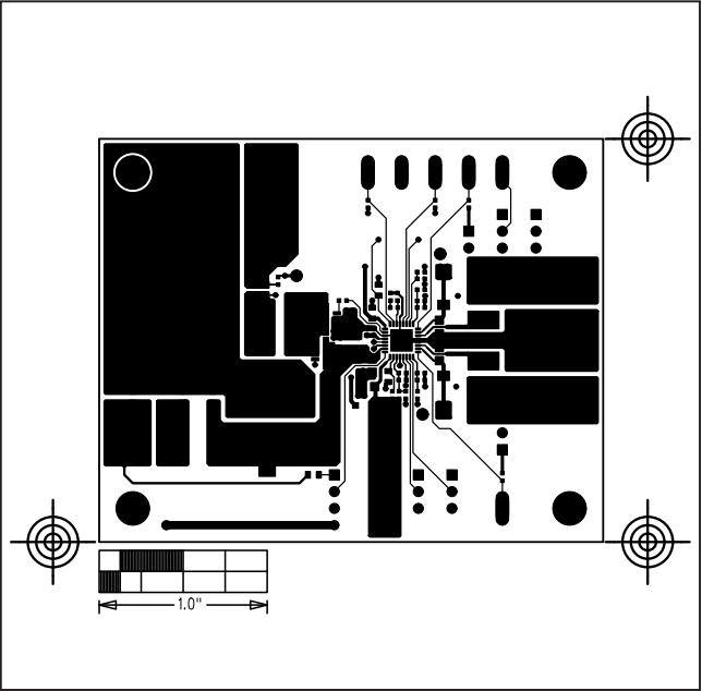
MAX20028 EV Kit PCB Layout—Component Side
