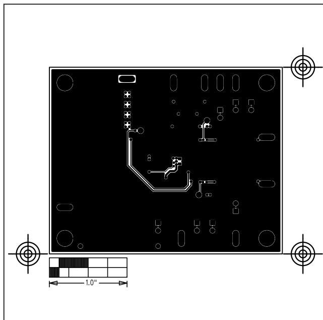
MAX20028 EV Kit PCB Layout—Solder Side
