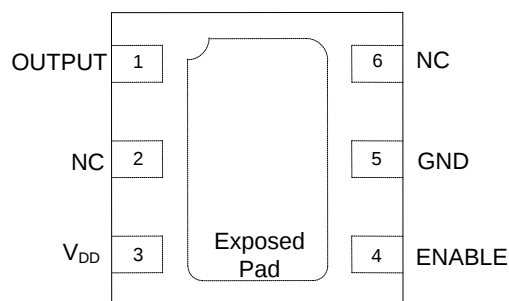
U-DFN2020-6
