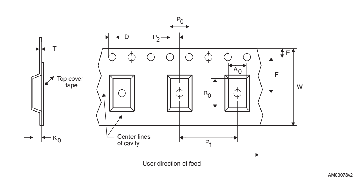
Figure 13. Carrier tape
