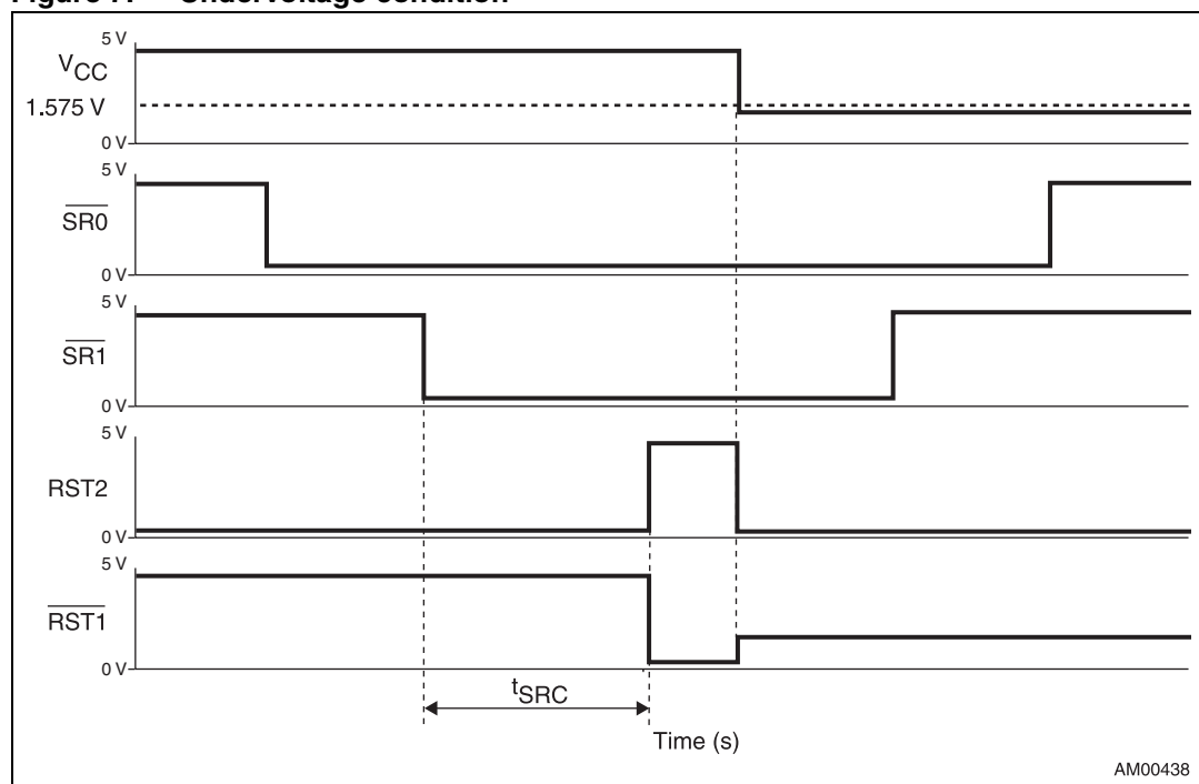
Figure 7. Undervoltage condition
