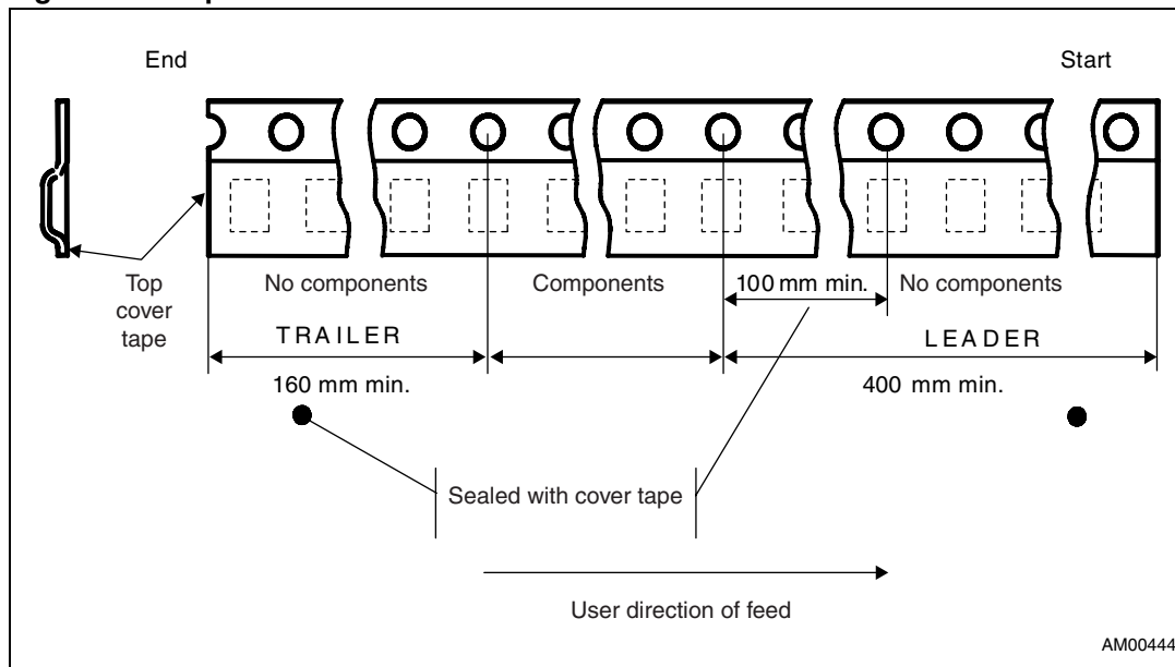
Figure 15. Tape trailer/leader
