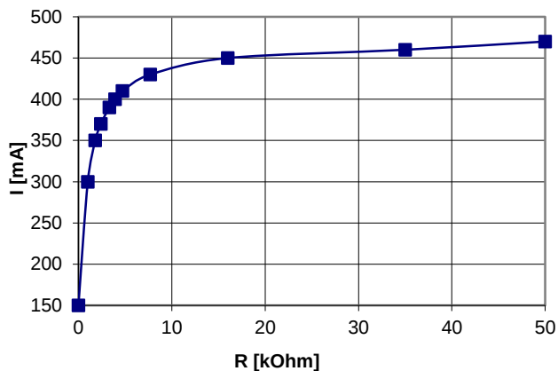
QPA3230 Current vs. external resistor
