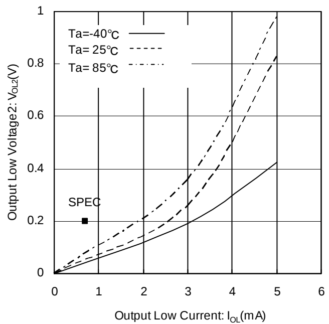
Fig 7. Output Low Voltage2 vs Output Low Current (V<sub>CC</sub>=1.6V)
