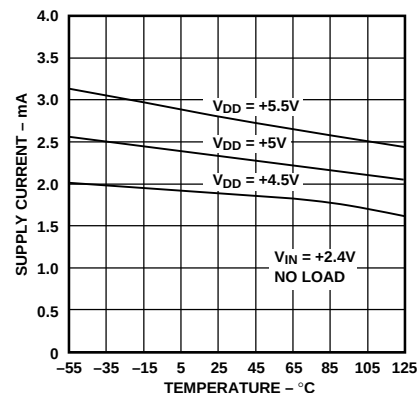
Figure 20. Supply Current vs. Temperature
