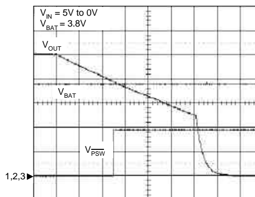
PSW Output Timing
