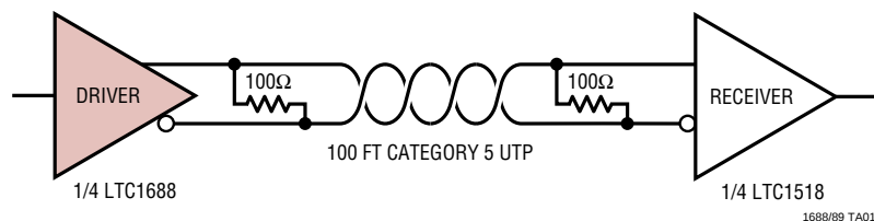
50Mbps RS485 Data Connection
