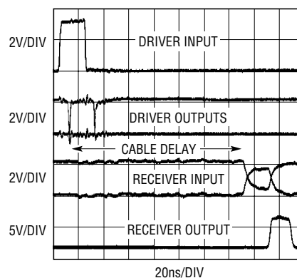
20ns Pulse Across 100 Feet of Category 5 UTP
