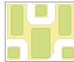
Figure 25. Solder stencil overlaid on ACMD-7602 bottom metal pattern
