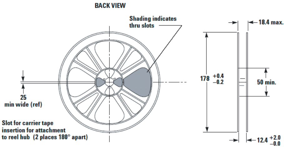
Figure 28. Reel drawing, back view
