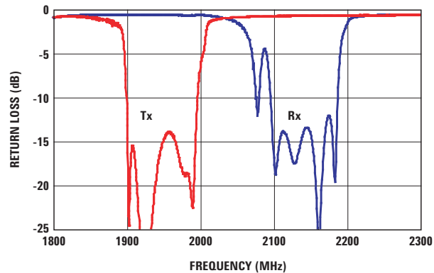
Figure 3. Tx and Rx port return loss
