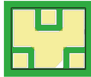
Figure 23. ACMD-7602 superposed on solder mask
