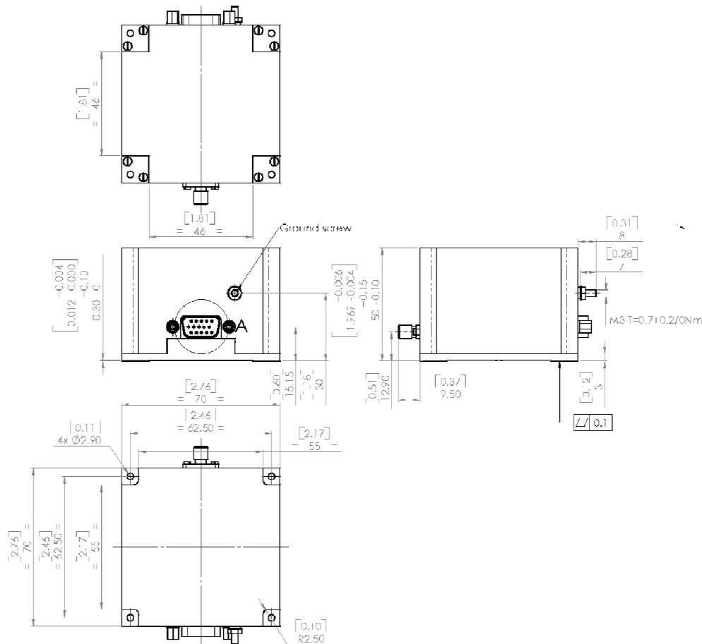
Figure 1 : Oscillator outline
