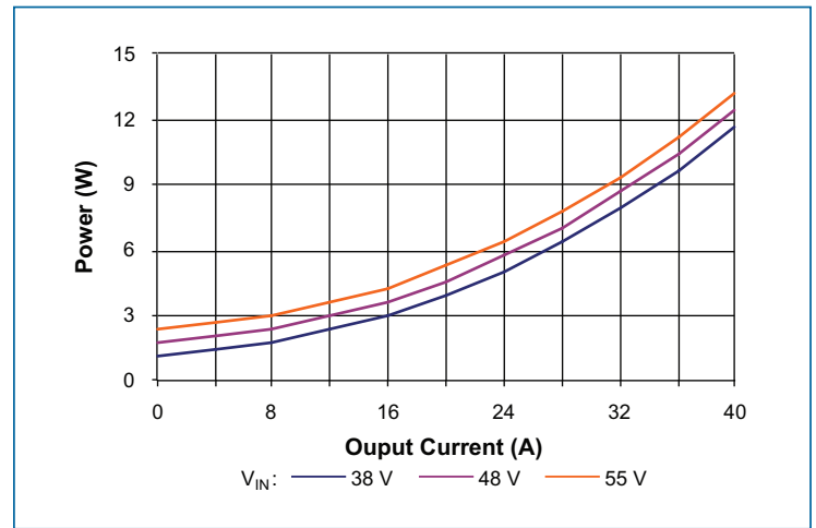
Figure 4 — Power dissipation vs. output current, 25°C ambient
