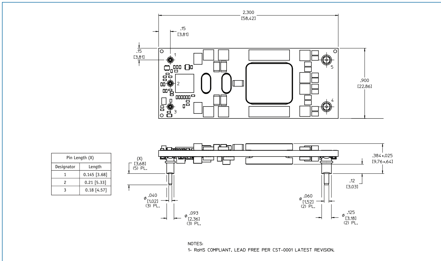
Figure 33 — IBC outline drawing
