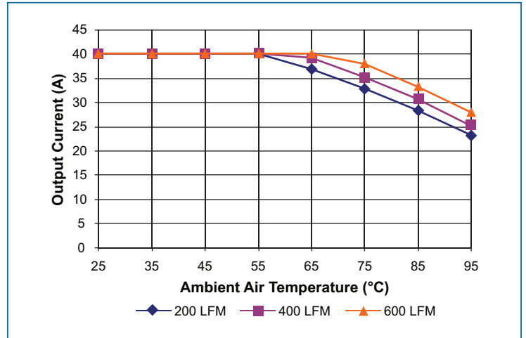
Figure 20 — Output current derating vs. ambient air temperature @ V_{IN} nominal. Longitudinal airflow. Board and junction temperatures within IPC-9592 derating guidelines
