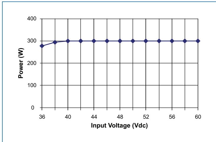
Figure 21 — Maximum output power vs. input voltage
