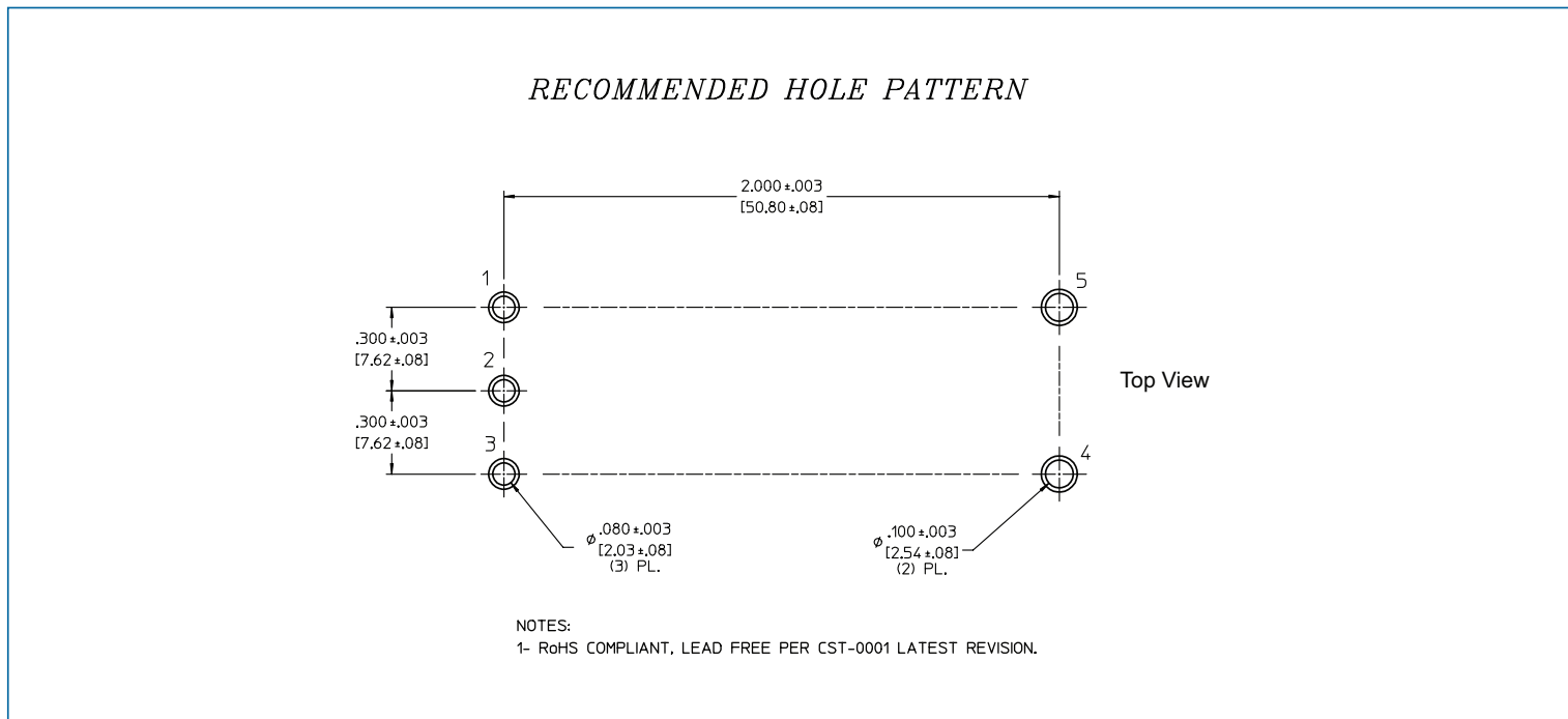
Figure 34 — IBC PCB recommended hole pattern
