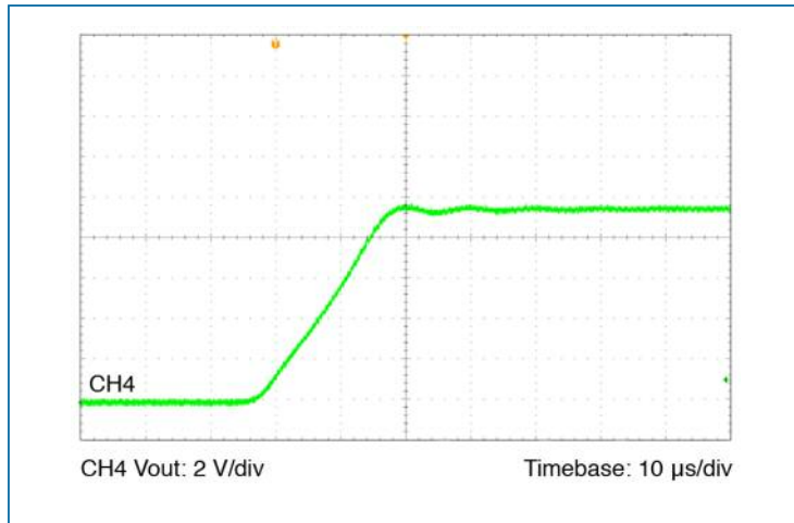
Figure 9 — Output voltage rise time at nominal line, 15% load
