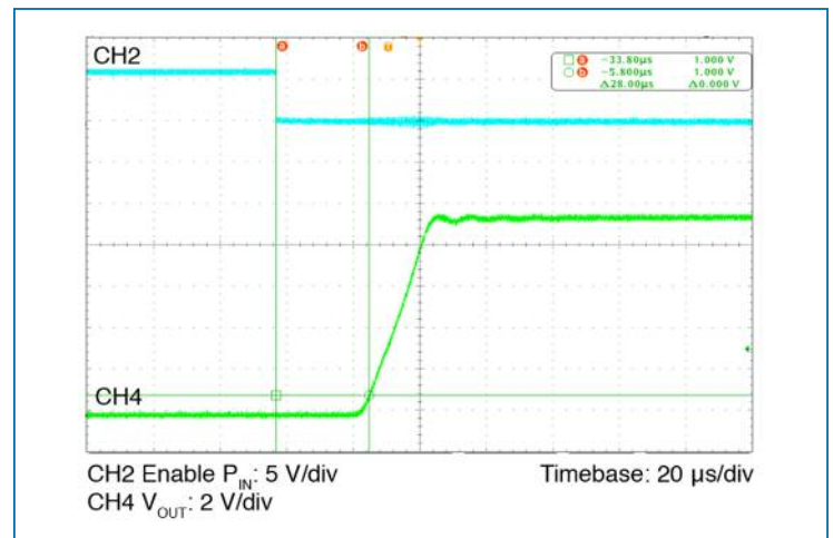
Figure 8 — Turn on delay time; Enable turn on delay at nominal line, 15% load. Also illustrates V_O Overshoot @ Turn-On.
