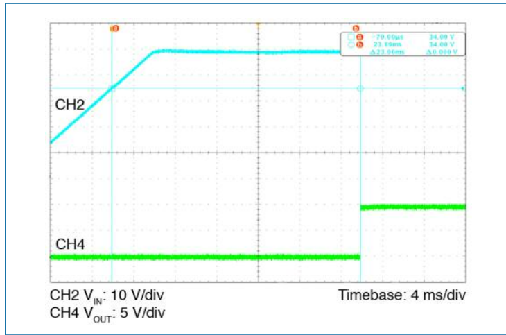
Figure 7 — Turn on delay time; V_{IN} turn on delay at nominal line, 15% load; Start-up inhibit time
