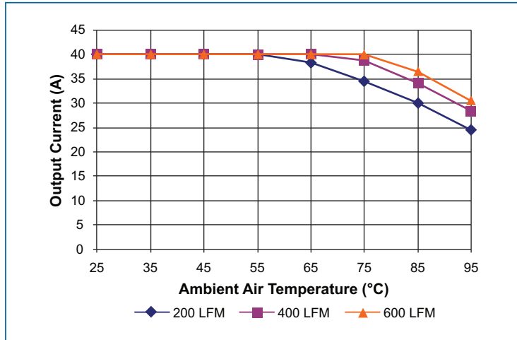
Figure 19 — Output current derating vs. ambient air temperature @ V_{IN} nominal. Transverse airflow. Board and junction temperatures within IPC-9592 derating guidelines
