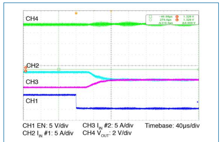
Figure 18 — Two modules parallel array test. V_{OUT} and I_{IN} change when one module is enabled. Nominal V_{IN} , I_{OUT} = 40 A
