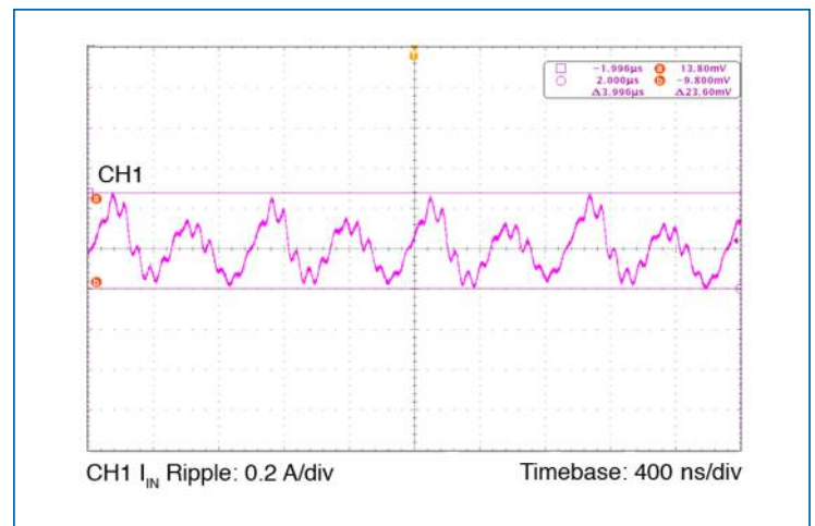
Figure 6 — Input reflected ripple current at nominal line, full load
