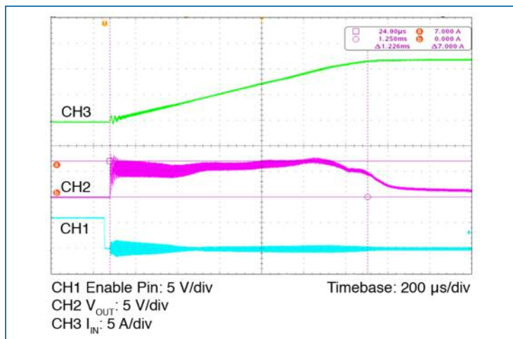
Figure 5 — Inrush current
