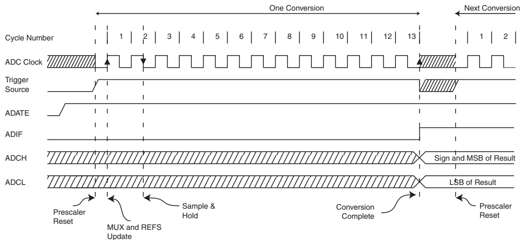
Figure 24-6. ADC Timing Diagram, Auto Triggerred Conversion
