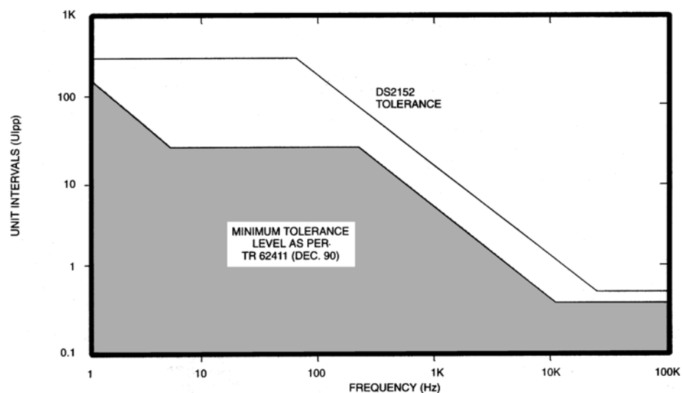
Figure 15-2. Jitter Tolerance
