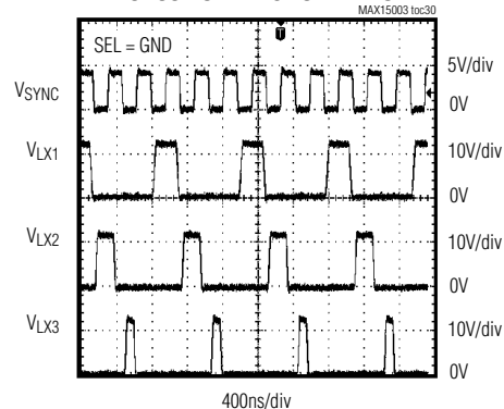
120° OUT-OF-PHASE OPERATION
