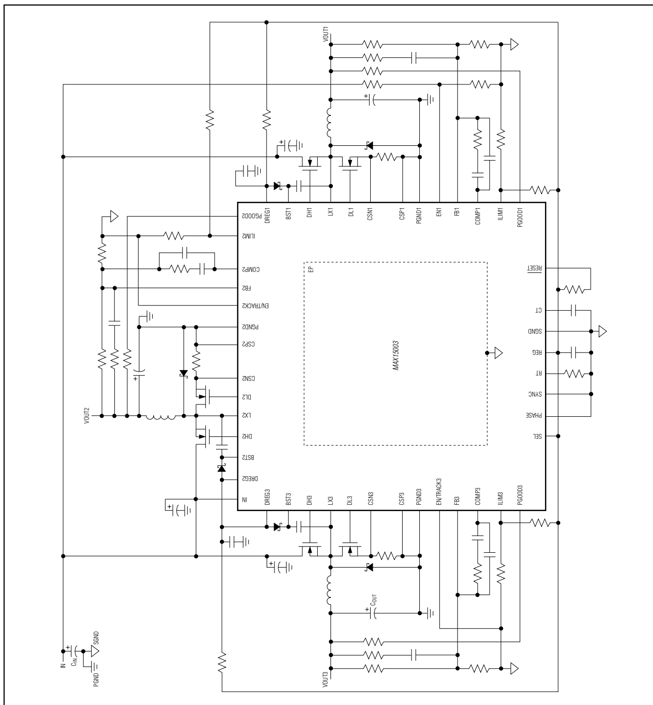
Figure 11. Ratiometric Triple Tracker with Accurate Valley-Mode Current Sense
