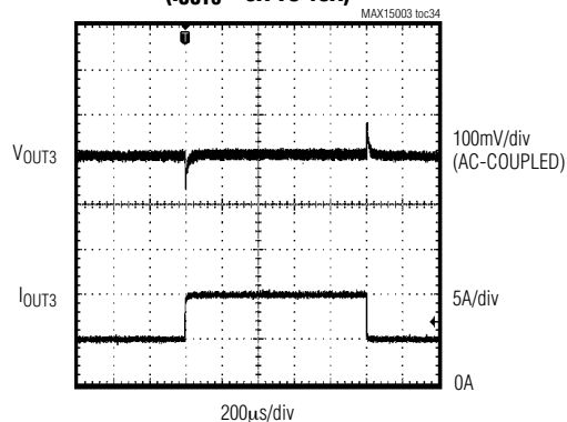
LOAD-TRANSIENT RESPONSE ( I_{OUT3} = 5A TO 10A )
