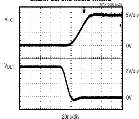
BREAK-BEFORE-MAKE TIMING
