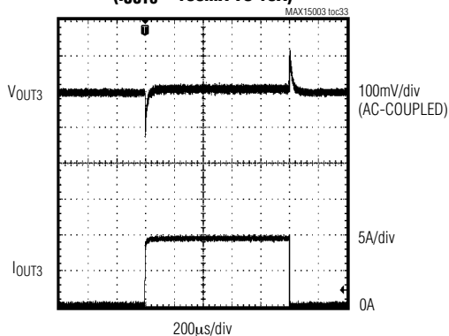
LOAD-TRANSIENT RESPONSE ( I_{OUT3} = 100mA TO 10A )
