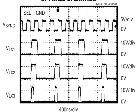
IN-PHASE OPERATION
