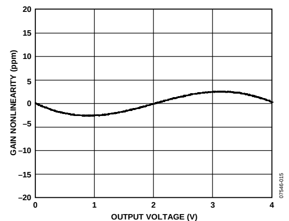
Figure 16. Gain Nonlinearity, R_L = 600\ \Omega , 2\ \text{k}\Omega , 10\ \text{k}\Omega
