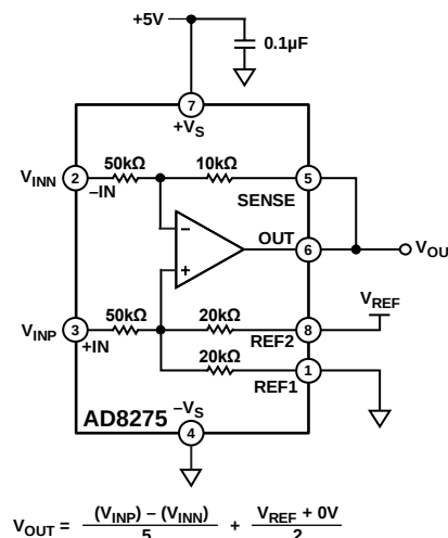
Figure 34. Basic Configuration 2: Split Reference
