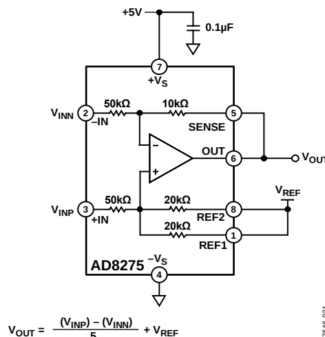
Figure 33. Basic Configuration 1: Shared Reference
