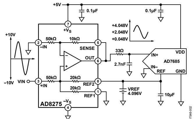
Figure 2. Translating \pm 10 V to 4.096 V ADC Full Scale
