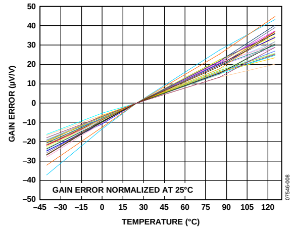
Figure 9. Gain Error vs. Temperature, Normalized at 25^\circ\text{C}
