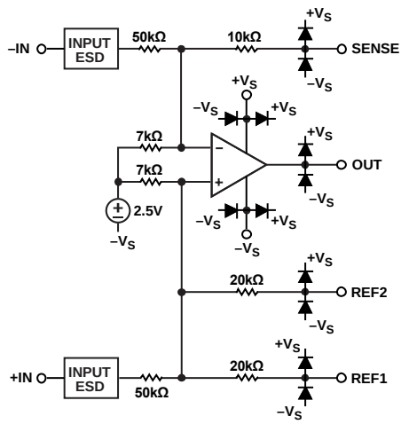
Figure 31. AD8275 Simplified Schematic
