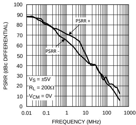
Figure 19. PSRR
