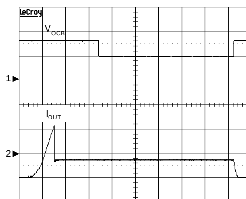
Ramped Load on Enabled Device
