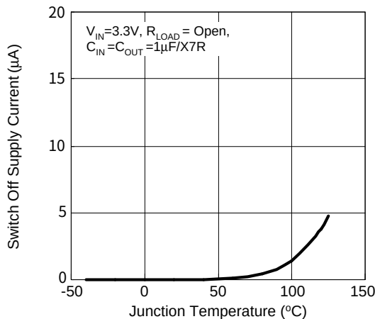
Switch Off Supply Current vs. Junction Temperature
