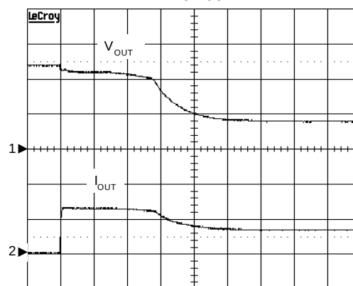
2.5W Load Connected to an Enabled Device
