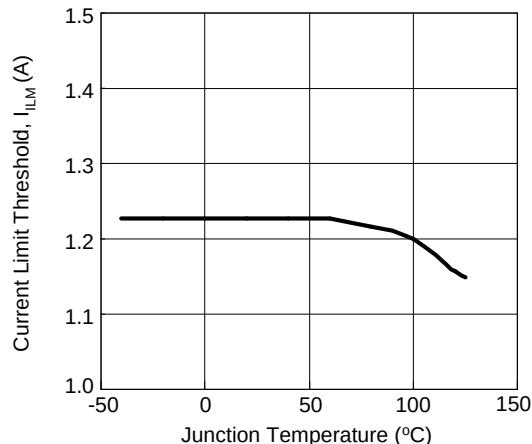
Current Limit Threshold vs. Junction Temperature
