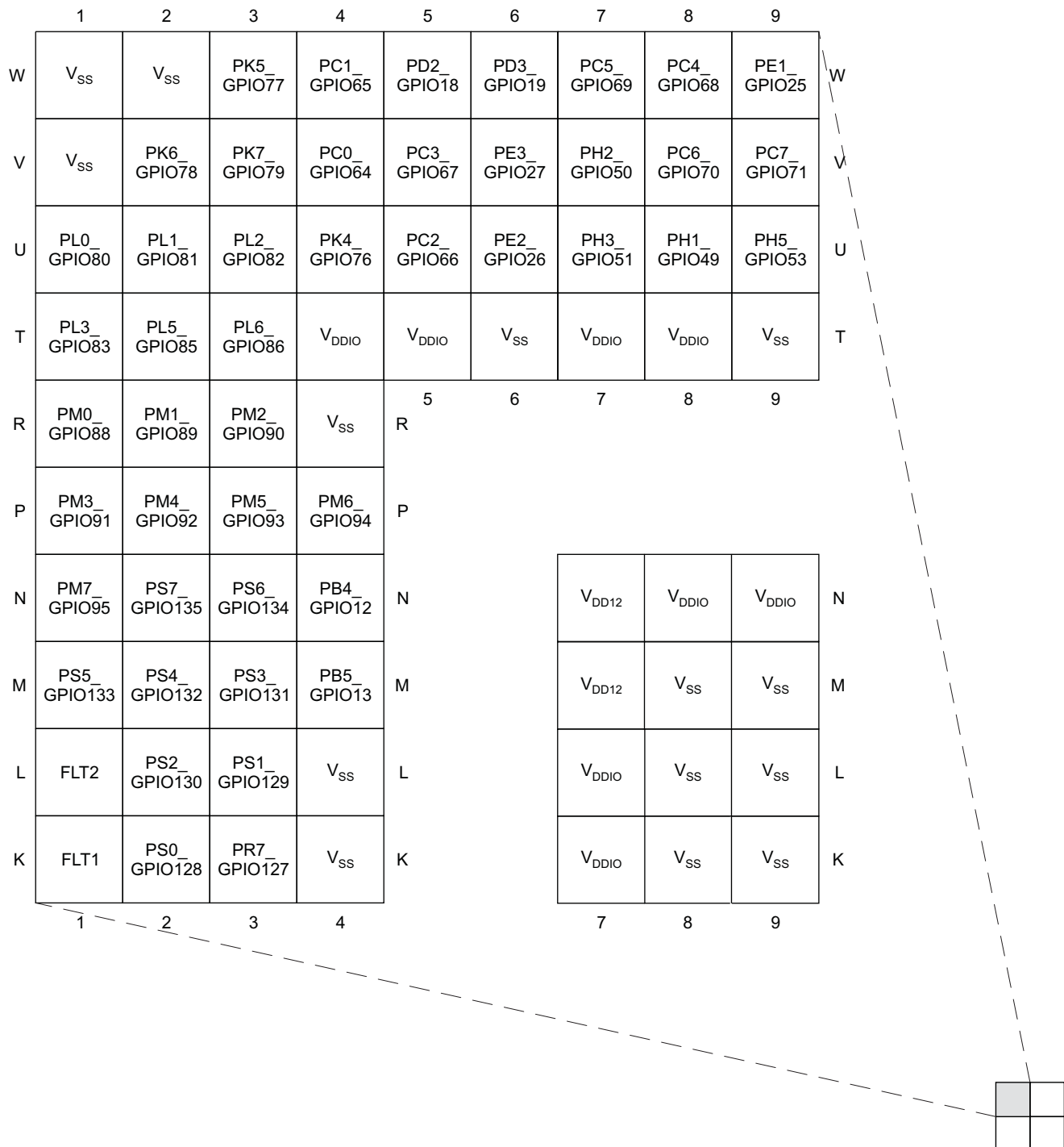
Figure 4-2. 289-Ball ZWT New Fine Pitch Ball Grid Array (Bottom View) – [Quadrant A]
