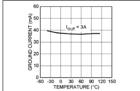
FIGURE 2-30: MIC2930x Ground Current vs. Temperature.
