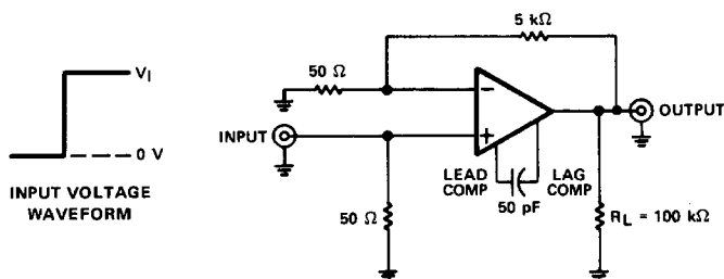
FIGURE 2—GAIN-OF-100 AMPLIFIER
