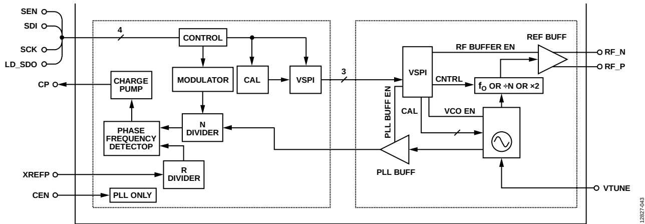
Figure 38. PLL and VCO Subsystems
