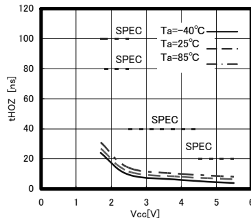
Fig.28 Time from HOLDB to output High-Z t_{HOZ}
