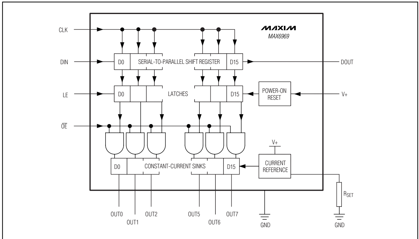
Figure 1. Block Diagram
