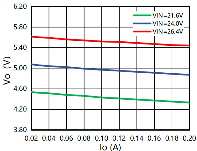
图3 输出电压 vs 输出电流 (VPS8701+VPT87FB-01B,24V to 5V/1W)
