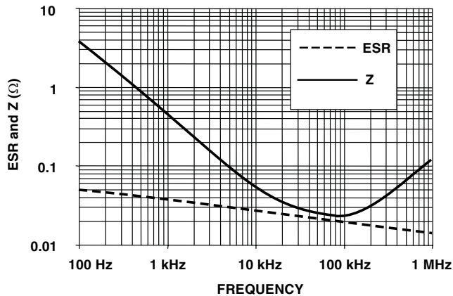
T97 330 \mu\text{F} - 6.3 V 'V' CASE SIZE ESR and Z vs. FREQUENCY
