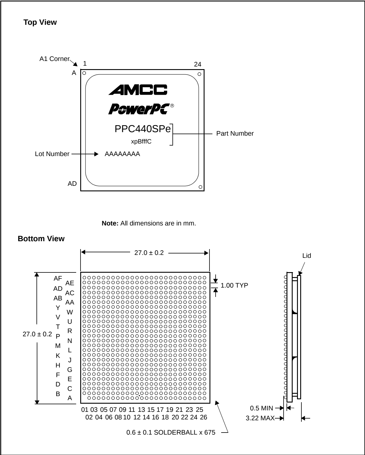
Figure 3. 27mm, 675-Ball FC-PBGA Core Package
