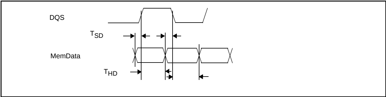
Figure 10. DDR SDRAM Memory Data and DQS
