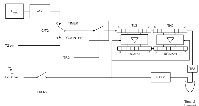
FIGURE 9: TIMER 2 IN CAPTURE MODE
