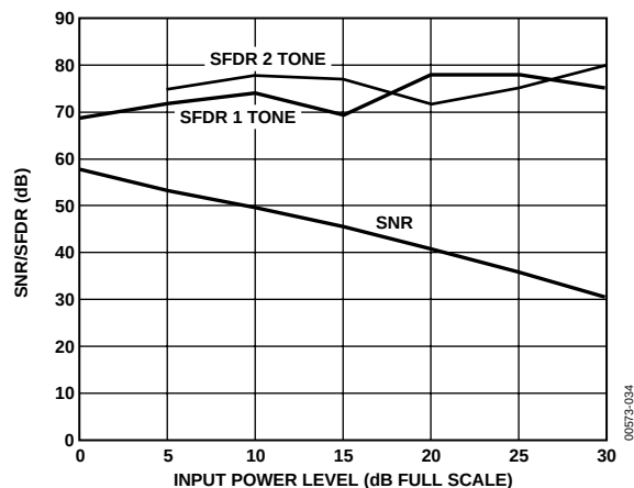
Figure 34. SNR/SFDR for IF @ 70 MHz (Clock = 40 MSPS)
