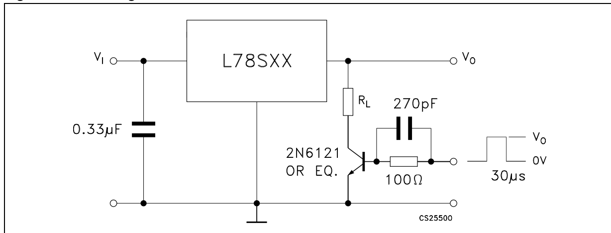
Figure 6. Load regulation
