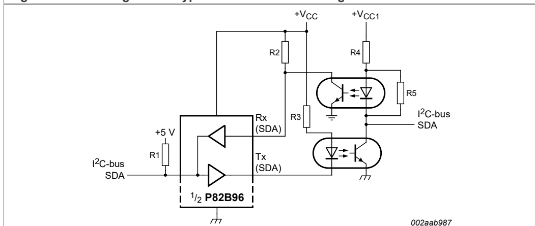
Figure 10. Galvanic isolation of I²C-bus nodes via opto-couplers
