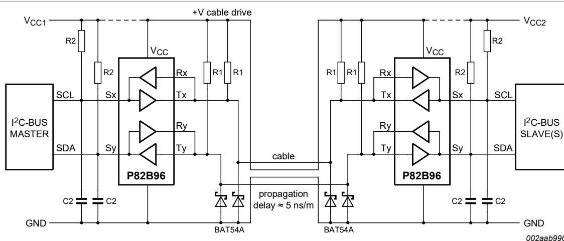
Figure 13. Driving ribbon or flat telephone cables
