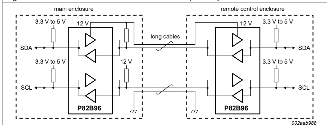
Figure 11. Long distance I²C-bus communications
