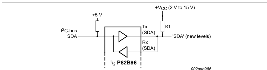
Figure 9. Interfacing an 'I²C' type of bus with different logic levels
