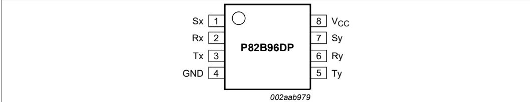
Figure 3. Pin configuration for TSSOP8
