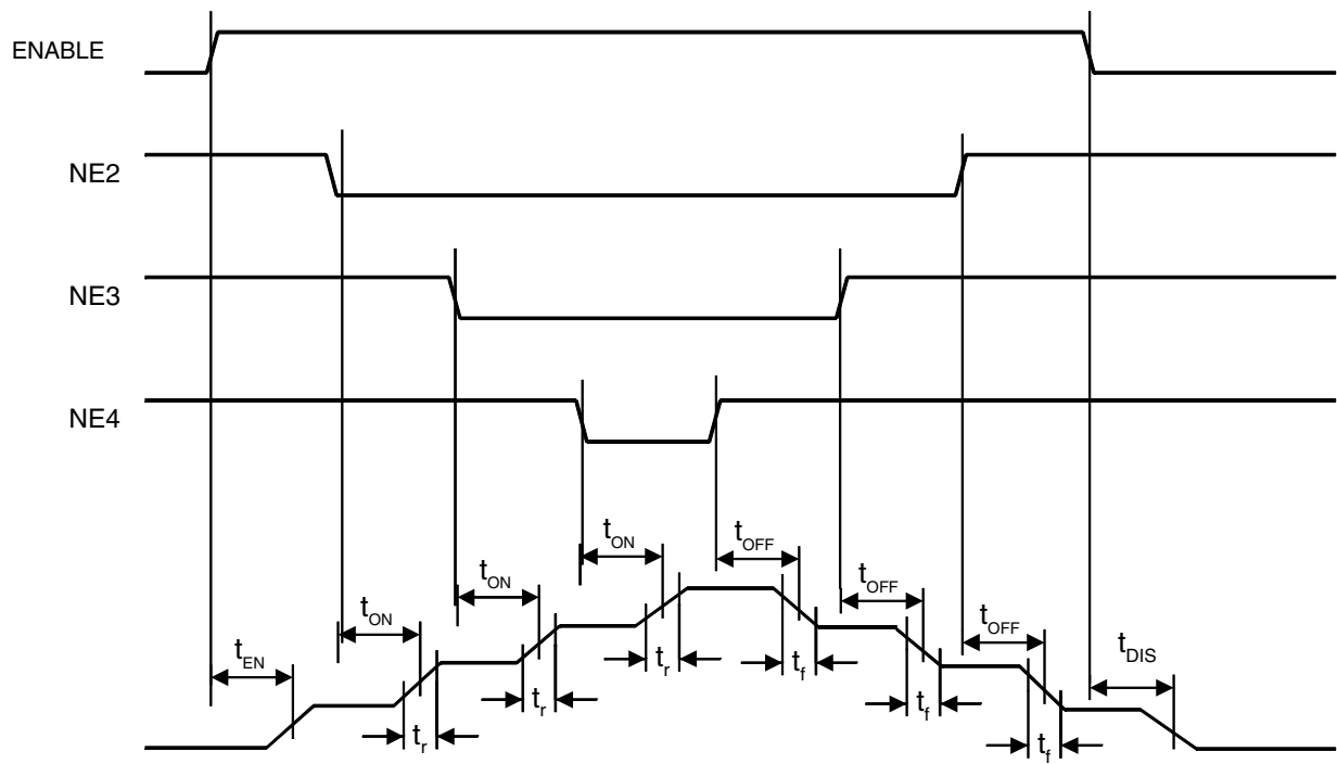
Figure 9-7. Timing Diagram
