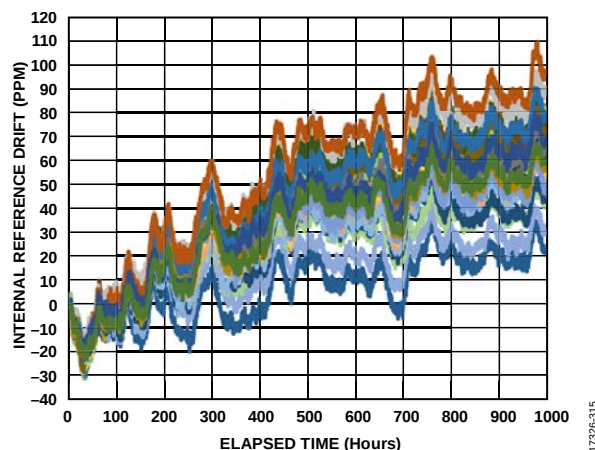
Figure 65. Reference Drift Through to 1000 Hours
