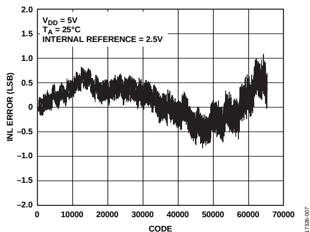
Figure 7. AD5679/AD5679R INL Error vs. Code
