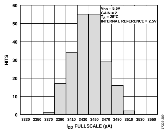
Figure 33. Supply Current ( I_{DD} ) Histogram with Internal Reference
