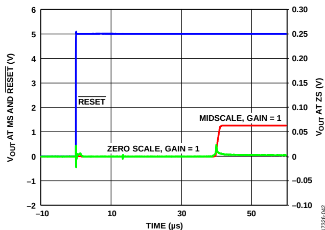
Figure 52. Hardware Reset
