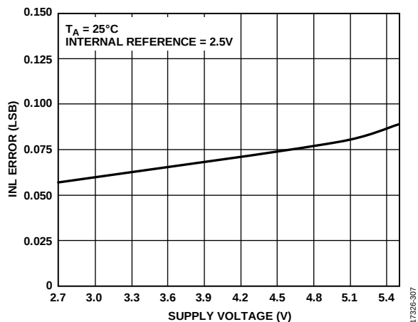
Figure 20. AD5674/AD5674R INL Error vs. Supply Voltage
