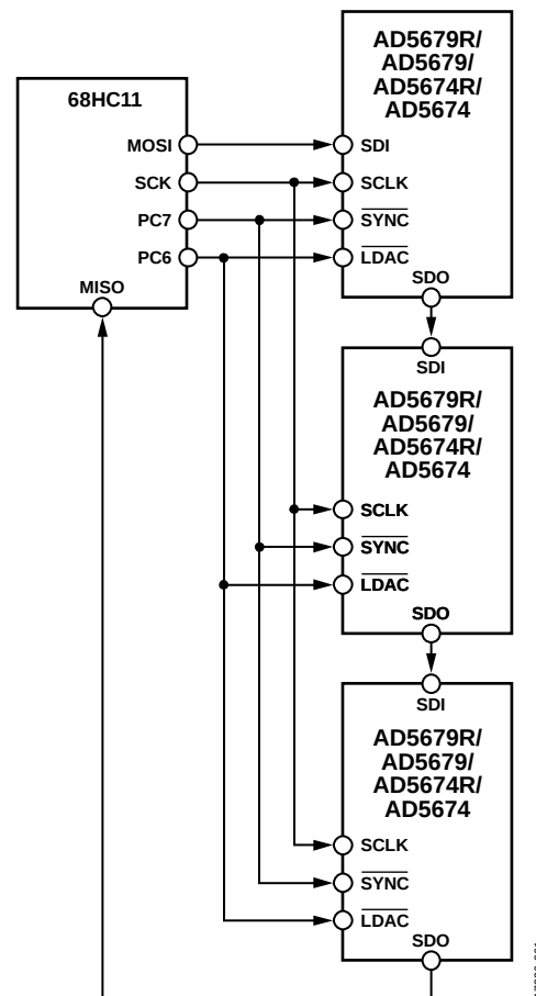
Figure 61. Daisy-Chaining the AD5674/AD5674R/AD5679/AD5679R to a Motorola® 68HC11
