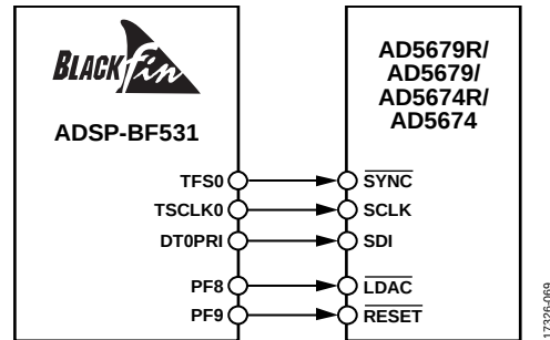
Figure 69. SPORT Interface
