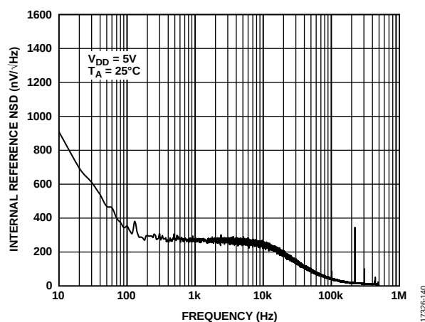
Figure 53. Internal Reference ND vs. Frequency
