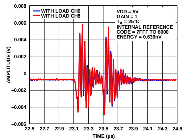
Figure 45. Digital-to-Analog Glitch Impulse
