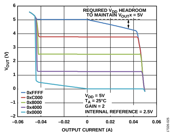
Figure 36. Source and Sink Capability at V_{DD} = 5V
