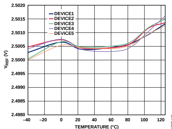
Figure 54. V_{REF} vs. Temperature
