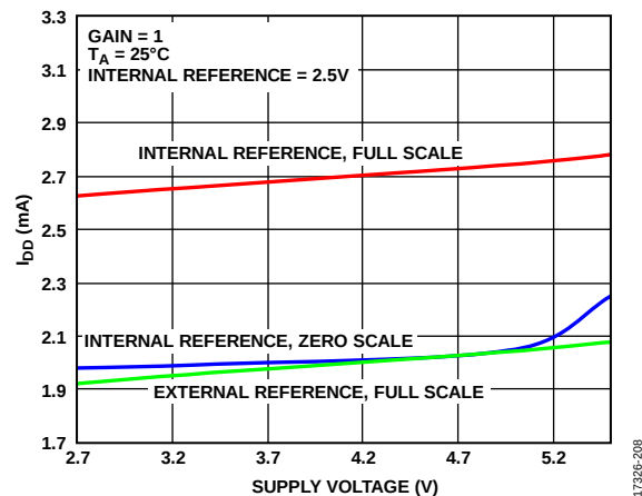
Figure 40. I_{DD} vs. Supply Voltage
