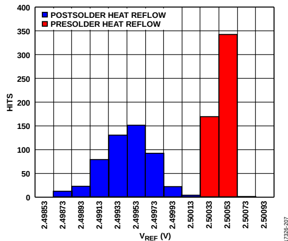
Figure 64. SHR Reference Voltage Shift
