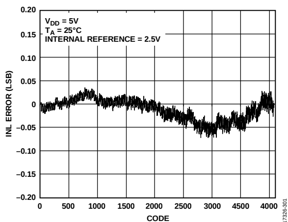
Figure 8. AD5674/AD5674R INL Error vs. Code
