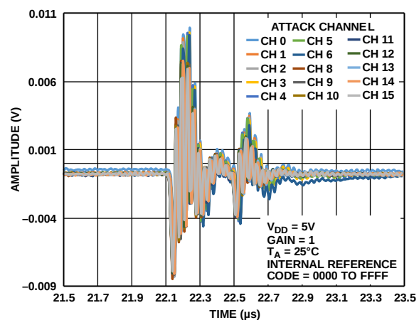
Figure 47. DAC-to-DAC Crosstalk
