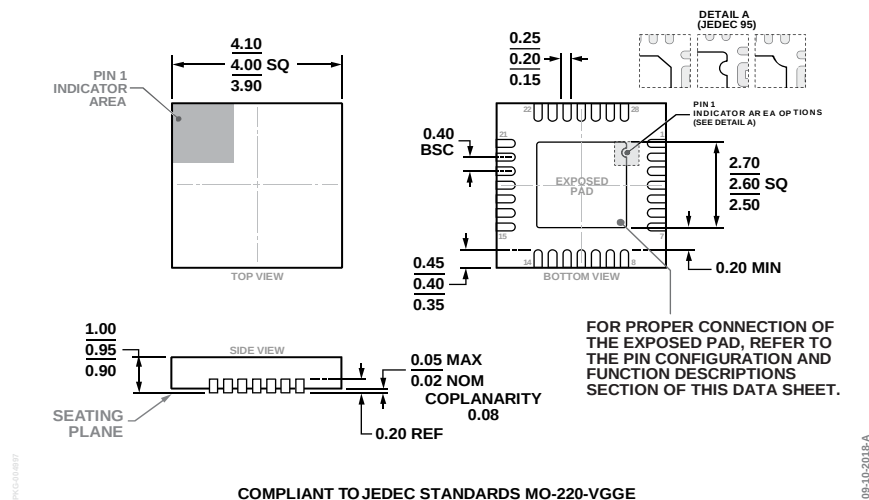
Figure 72. 28-Lead Lead Frame Chip Scale Package [LFCSP] 4 mm × 4 mm Body and 0.95 mm Package Height (CP-28-9)
