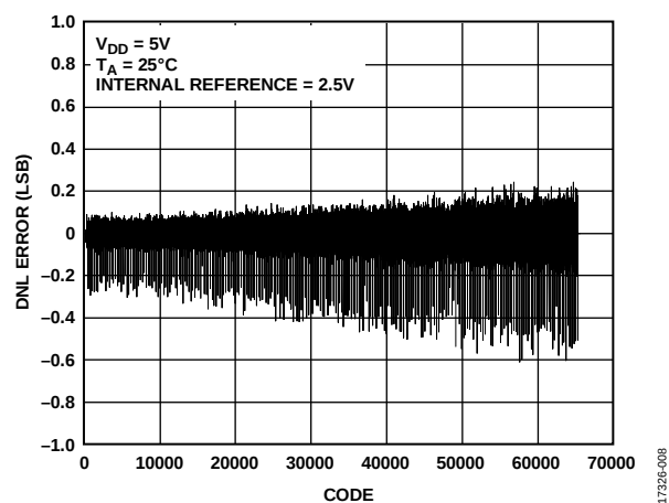
Figure 9. AD5679/AD5679R DNL Error vs. Code
