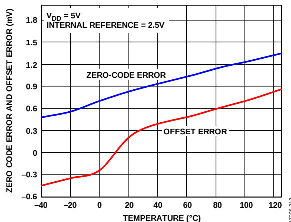
Figure 30. AD5674/AD5674R Zero Code Error and Offset Error vs. Temperature
