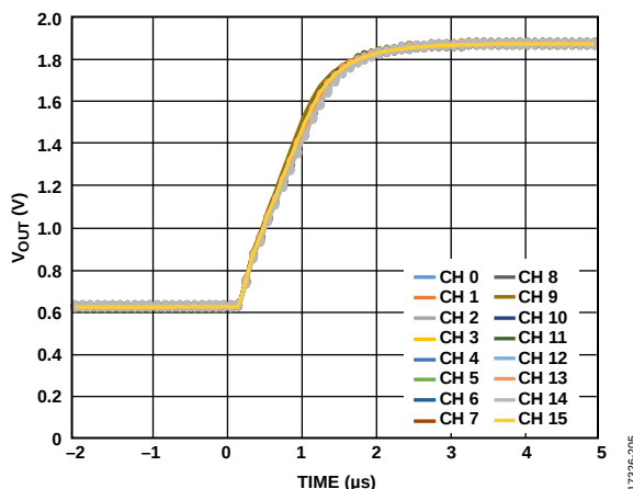
Figure 42. Settling Time
