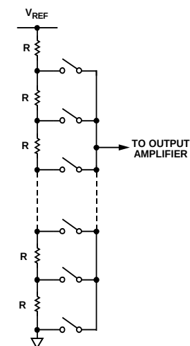
Figure 58. Resistor String Structure
