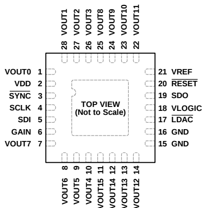
Figure 6. Pin Configuration
