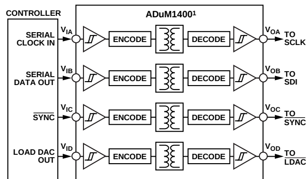
Figure 71. Isolated Interface
