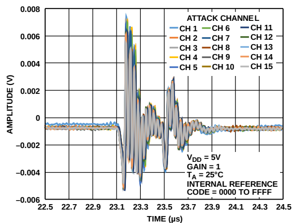
Figure 46. Analog Crosstalk
