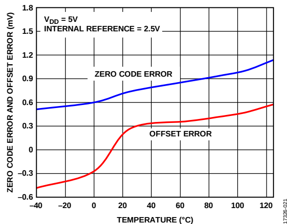
Figure 29. AD5679/AD5679R Zero Code Error and Offset Error vs. Temperature
