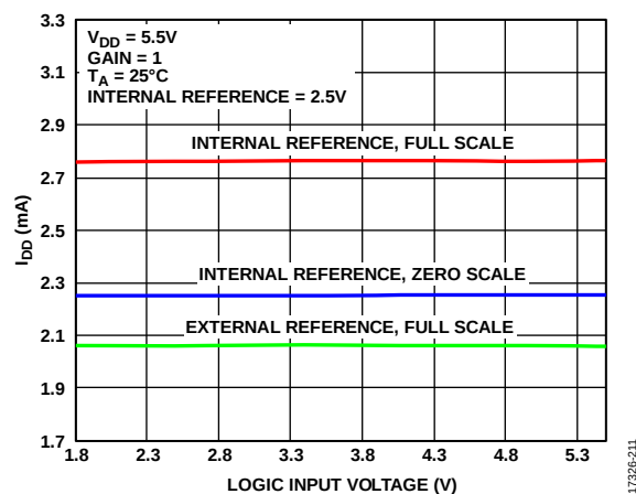
Figure 41. I_{DD} vs. Logic Input Voltage
