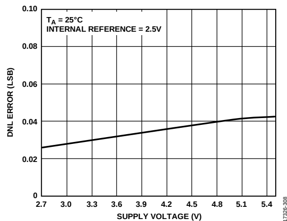
Figure 22. AD5674/AD5674R DNL Error vs. Supply Voltage
