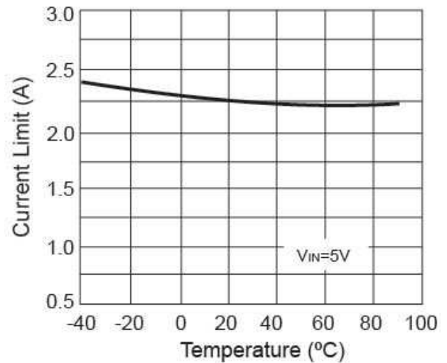
Figure 6. Current Limit vs. Temperature
