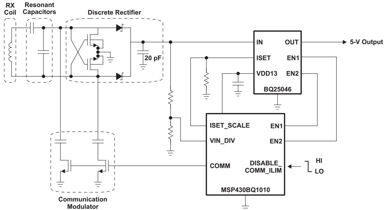
Figure 1. Application Schematic
