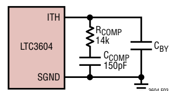
Figure 3. Compensation Components
