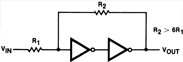
Figure 3. Schmitt Trigger
