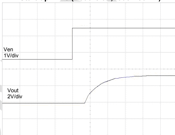
Start-up Time ( V_{out}=3.3V , I_{out}=150mA )
