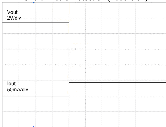
Short Circuit Protection ( V_{out}=3.3V )
