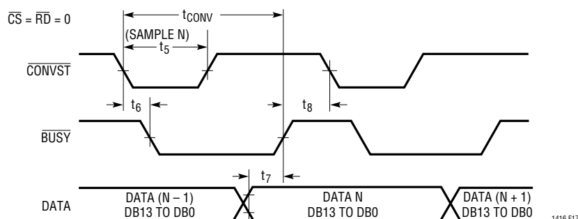
Figure 17. Mode 1a. \overline{\text{CONVST}} Starts a Conversion. Data Outputs Always Enabled ( \text{CONVST} = \square\square\square )
