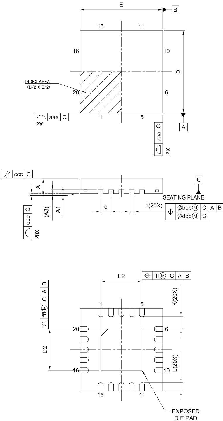
Figure 2.2 HWQFN 20-pin
