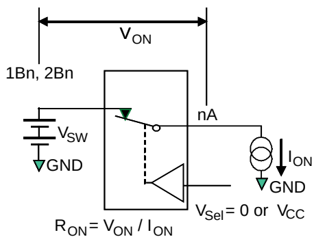
Figure 3. On Resistance
