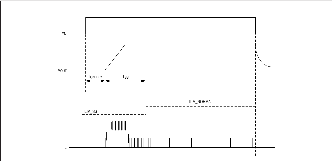
Figure 3. Soft-Start
