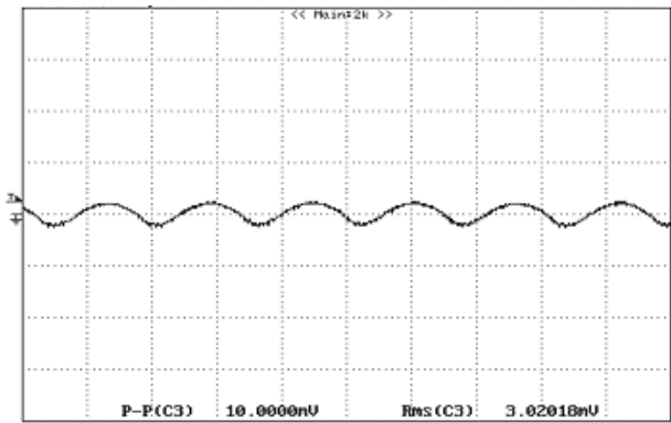
Figure 8: Output ripple & noise at 12Vin, 0.9V/6A out
