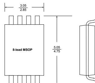
Figure 2. Package Type
