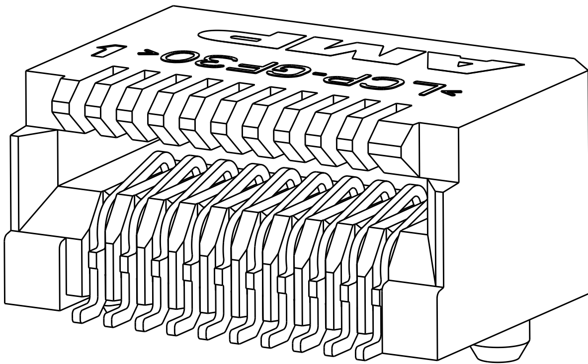
1888247-1,2,3,4,5 AS SHOWN
