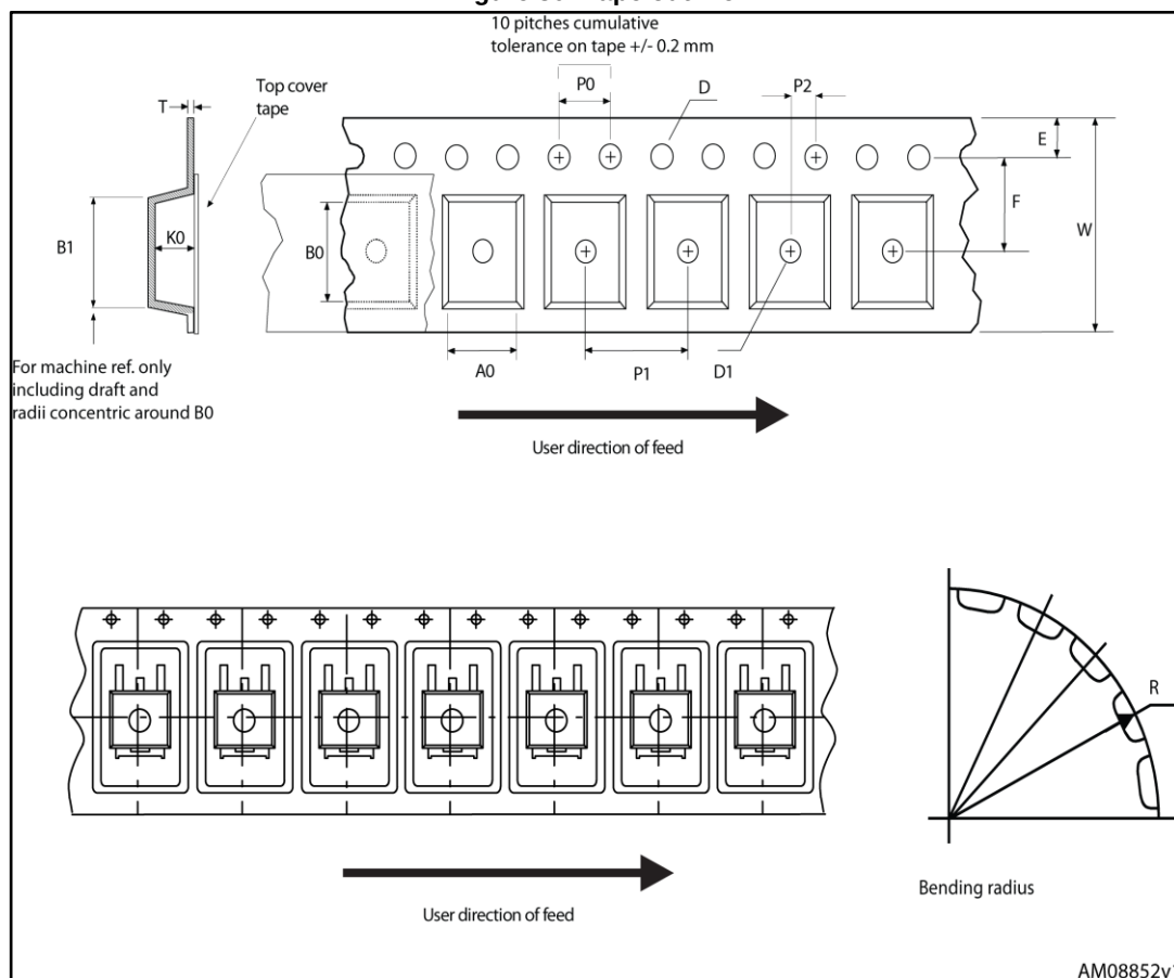
Figure 30: Tape outline
