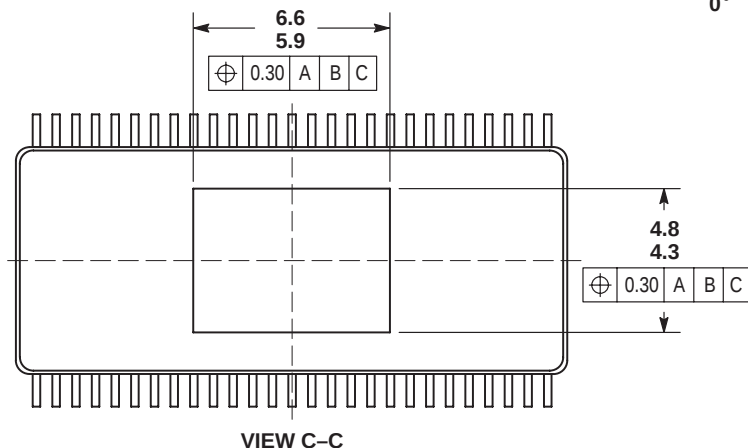
VIEW C-C
